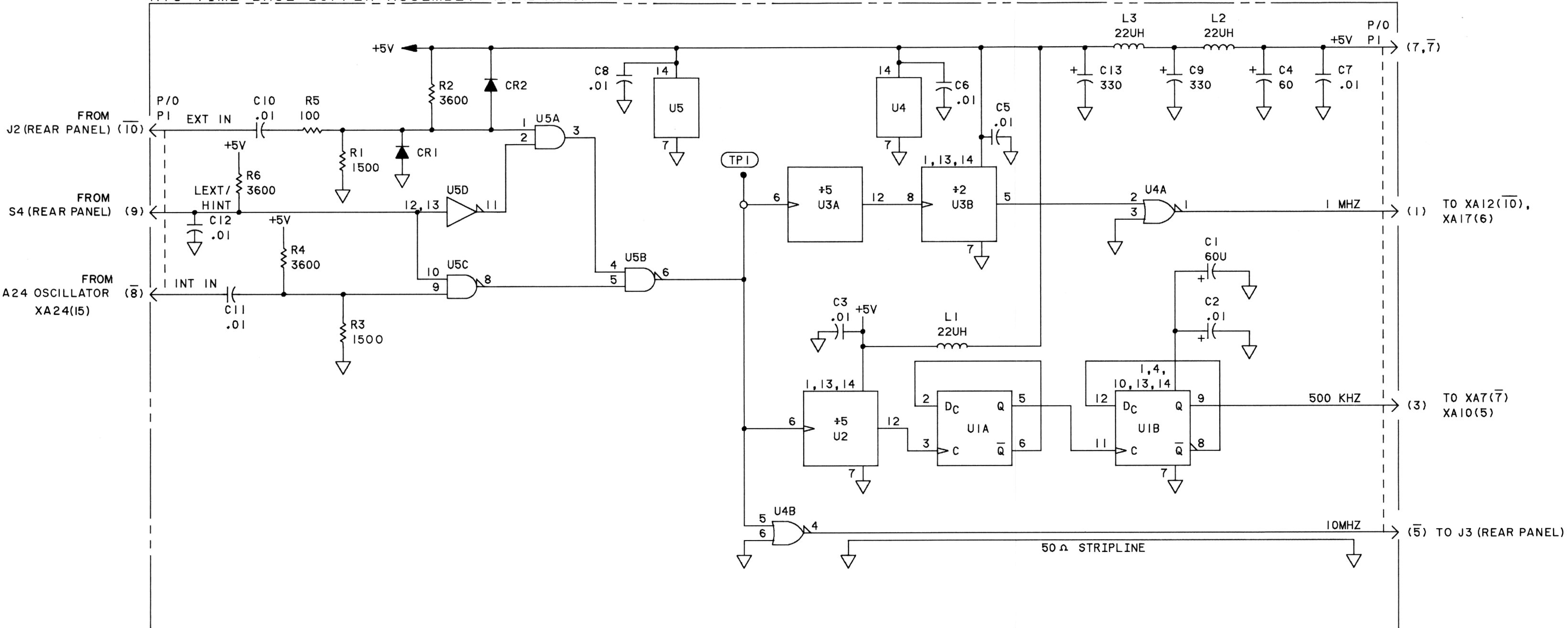
Figure 8-42. A18 Time Base Buffer Assembly
