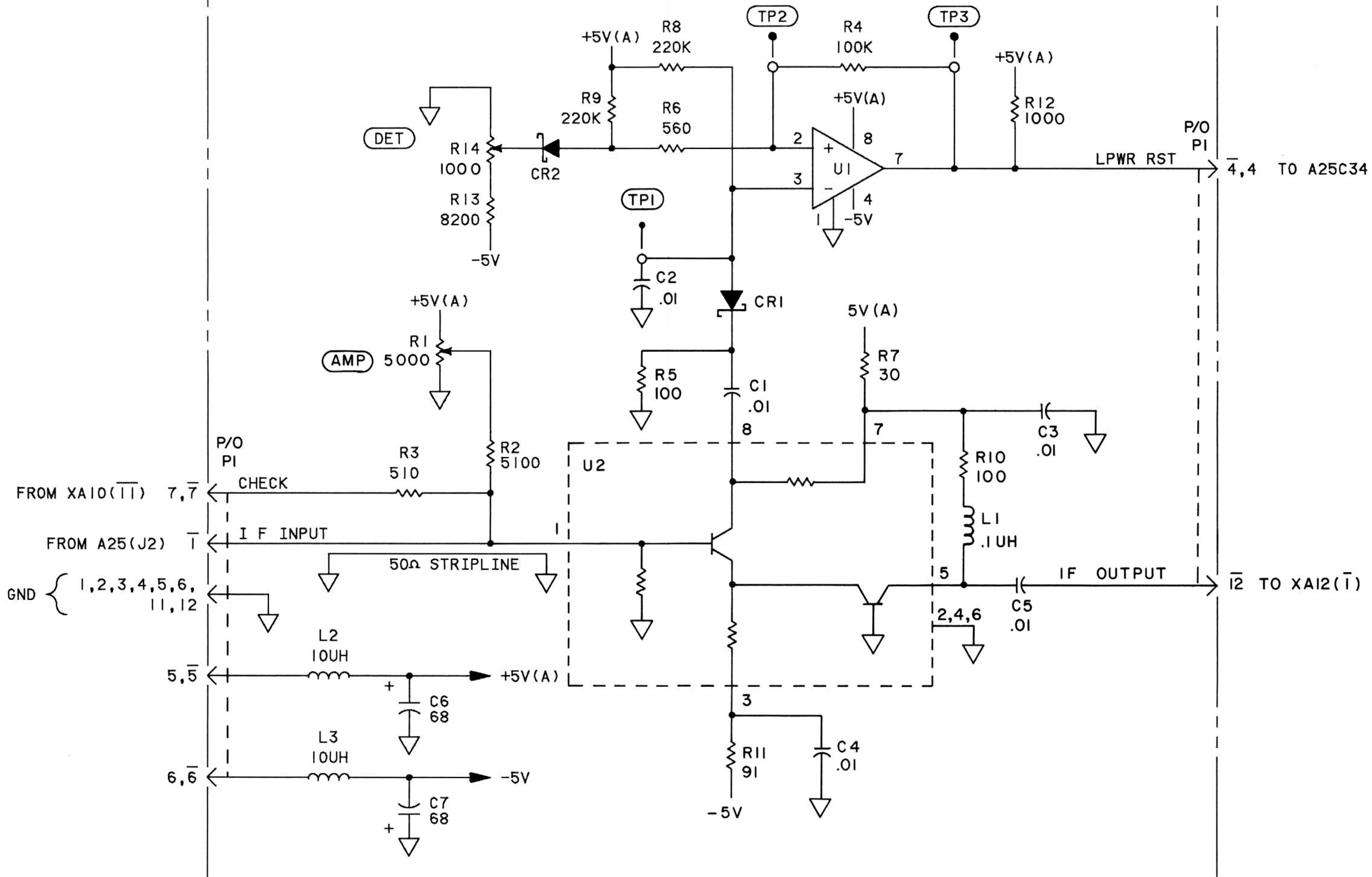
Figure 8-34. A11 IF Limiter Assembly
