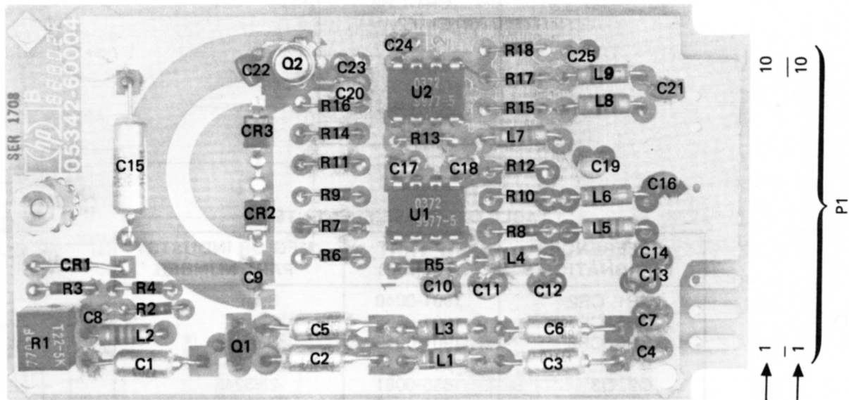
Part of Figure 8-27. A4 Offset VCO Assembly
