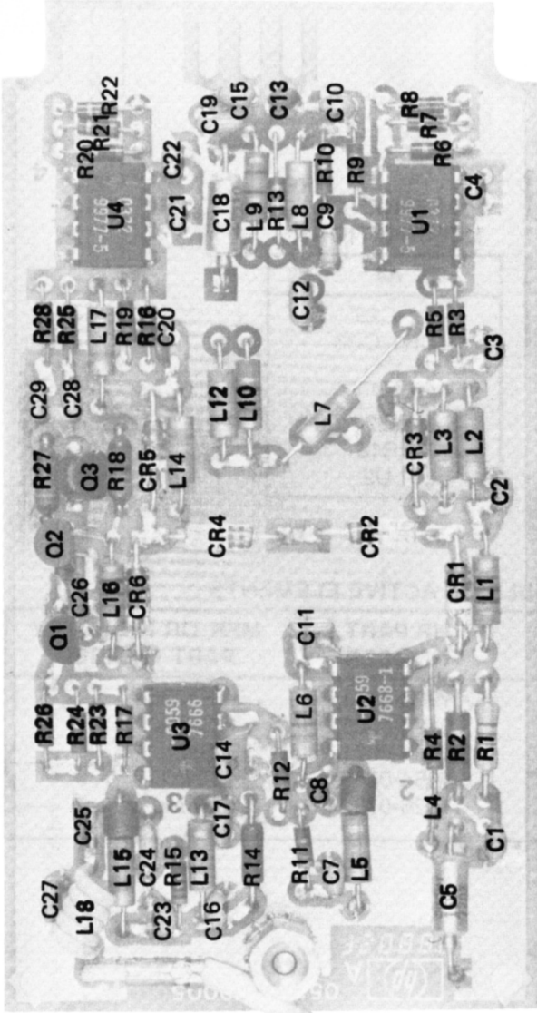
Part of Figure 8-28. A5 RF Multiplexer Assembly
