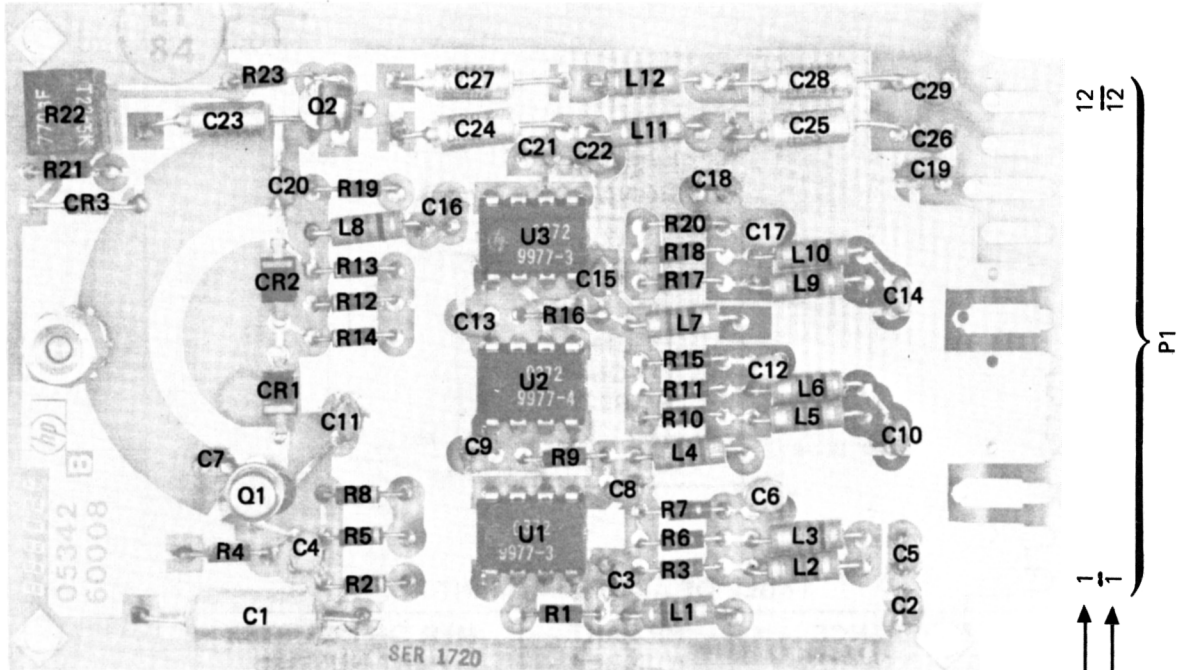
Part of Figure 8-31. A8 Main VCO Assembly
