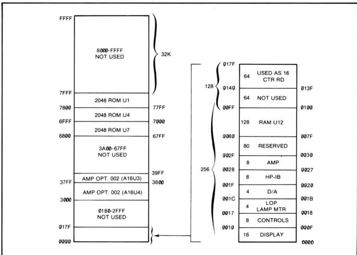
Figure 8-15. Memory Arrangement
