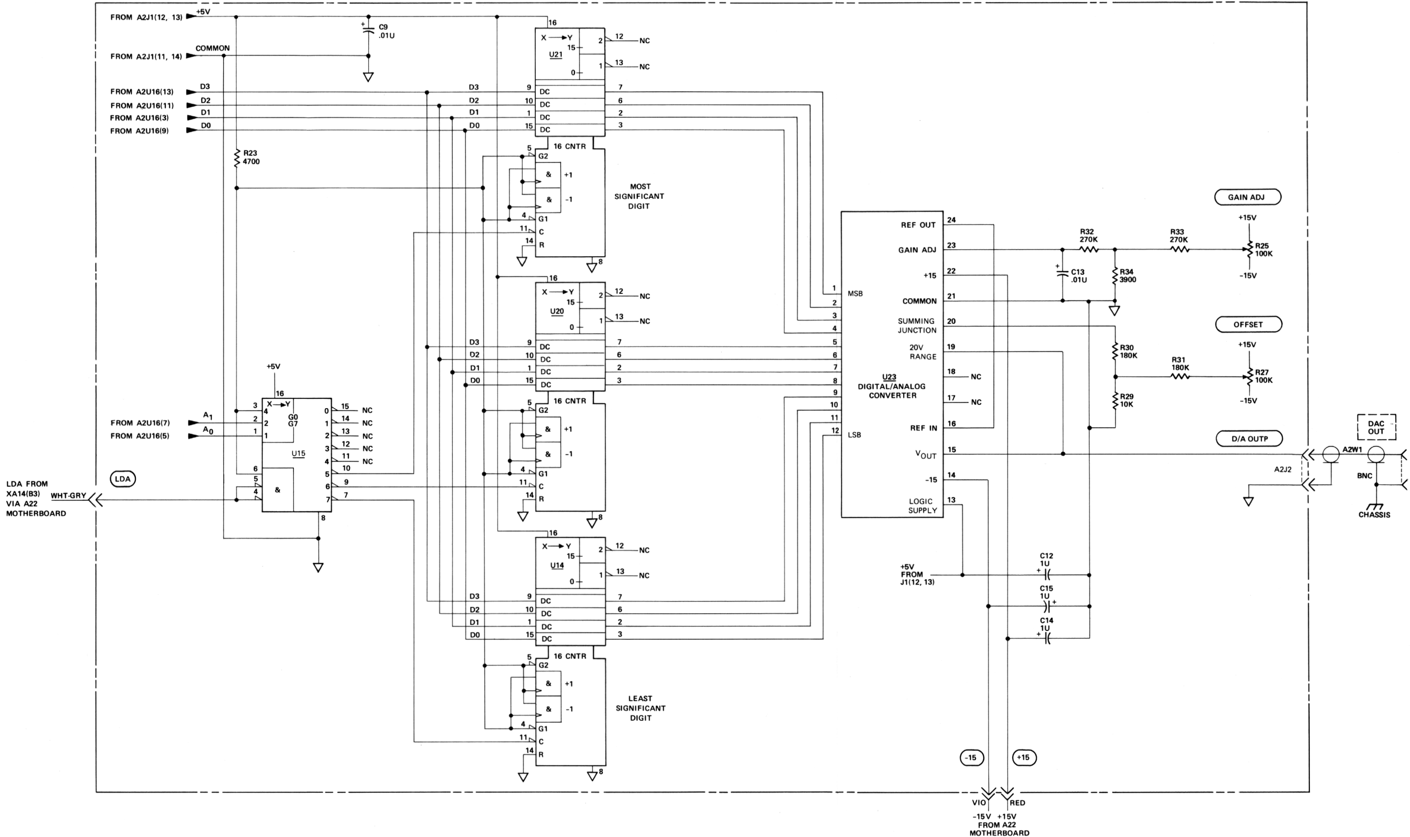
A2 DISPLAY DRIVER ASSEMBLY (05342-60028) ADDITIONS FOR OPTION 004
