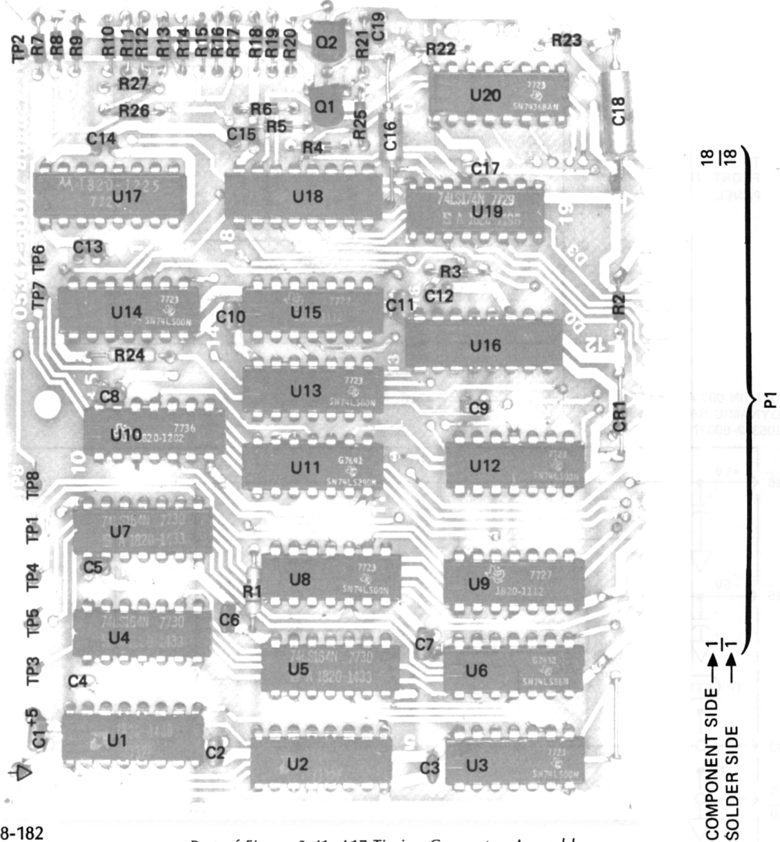
Part of Figure 8-41. A17 Timing Generator Assembly
