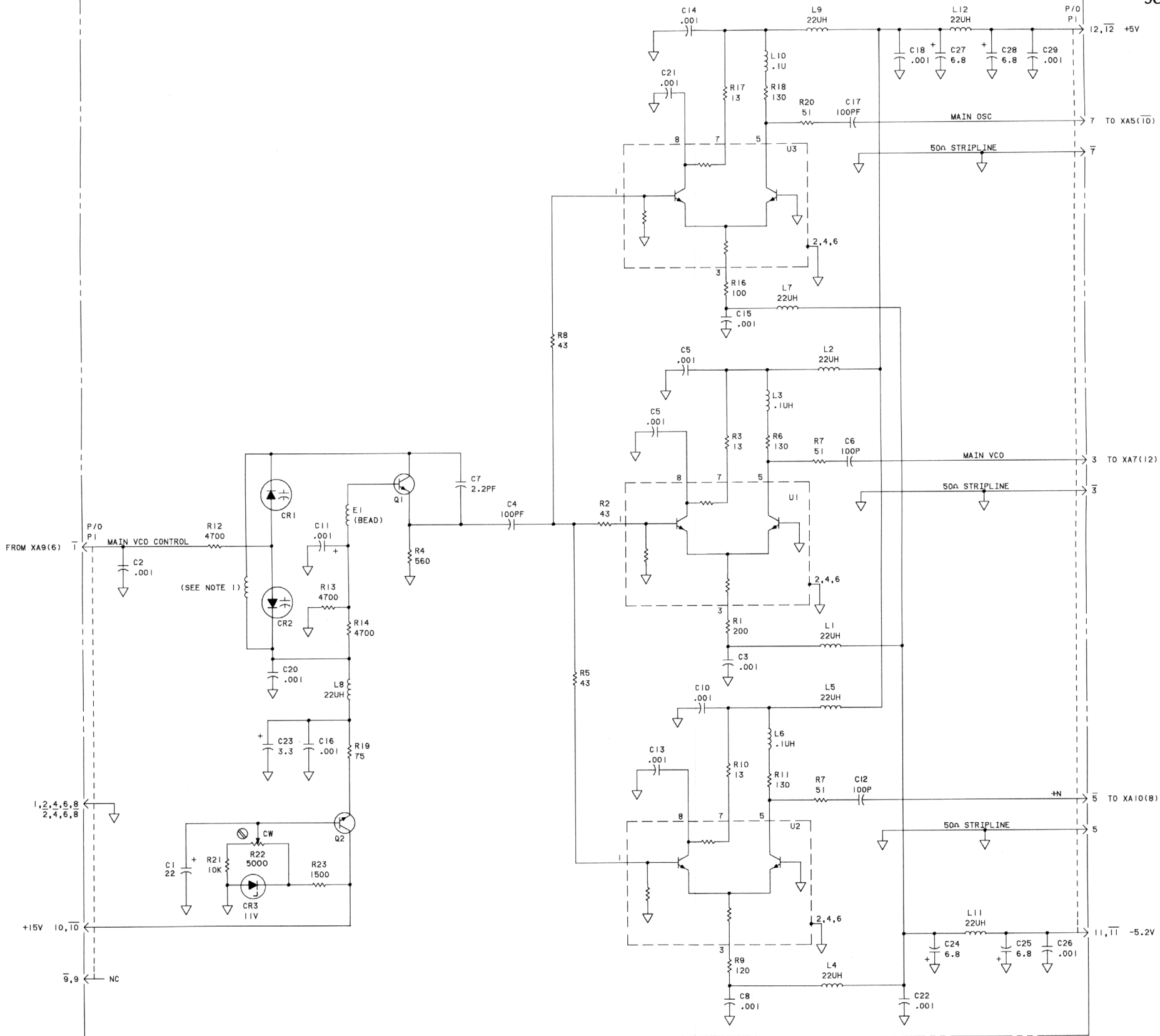
Figure 8-31. A8 Main VCO Assembly
