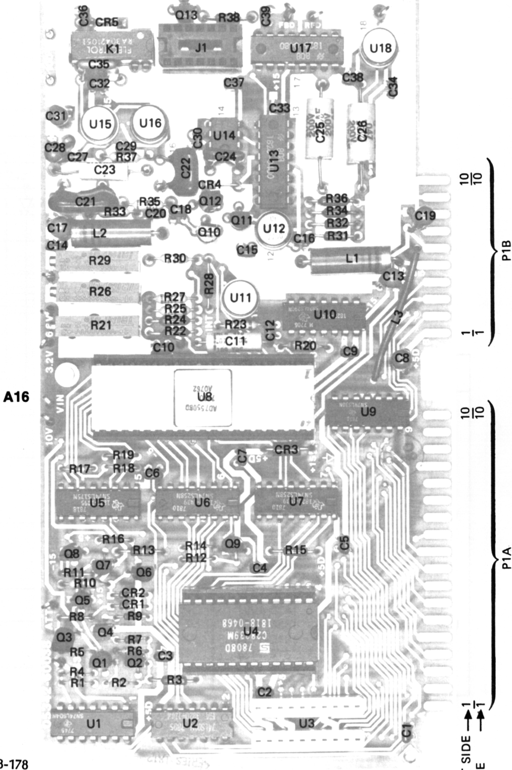
Part of Figure 8-39. Option 002 A16 Amplitude Measurements, A27 Low Frequency Amplifier, and U2 High Frequency Amplifier Assemblies
