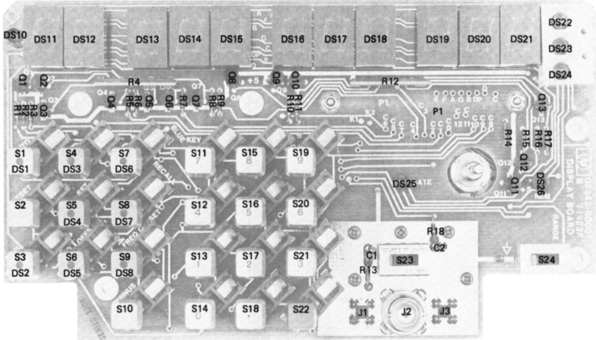
Part of Figure 8-24. A1 Display Assembly and A2 Display Drive Assembly
