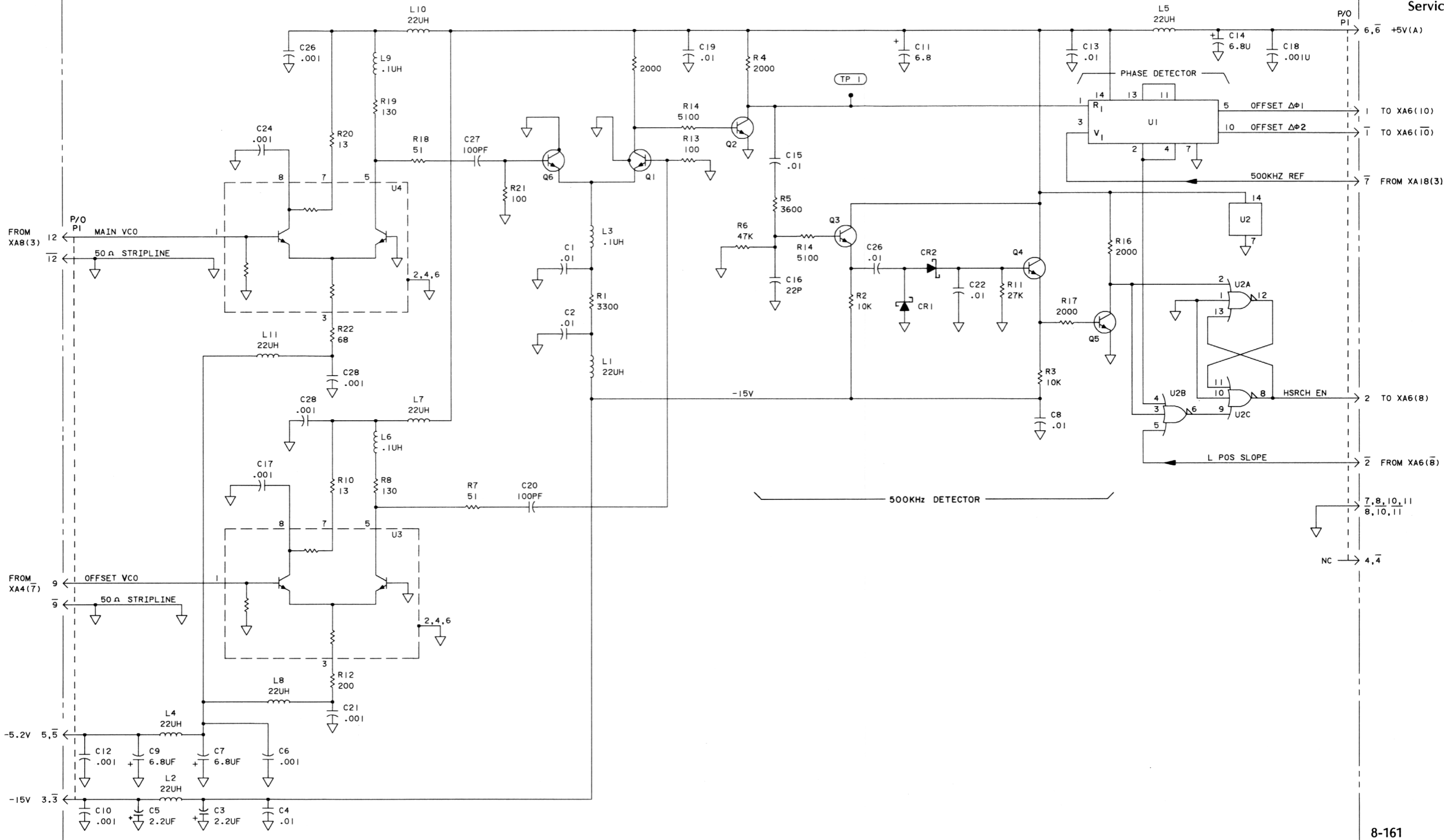
Figure 8-30. A7 Mixer/Search Control Assembly
