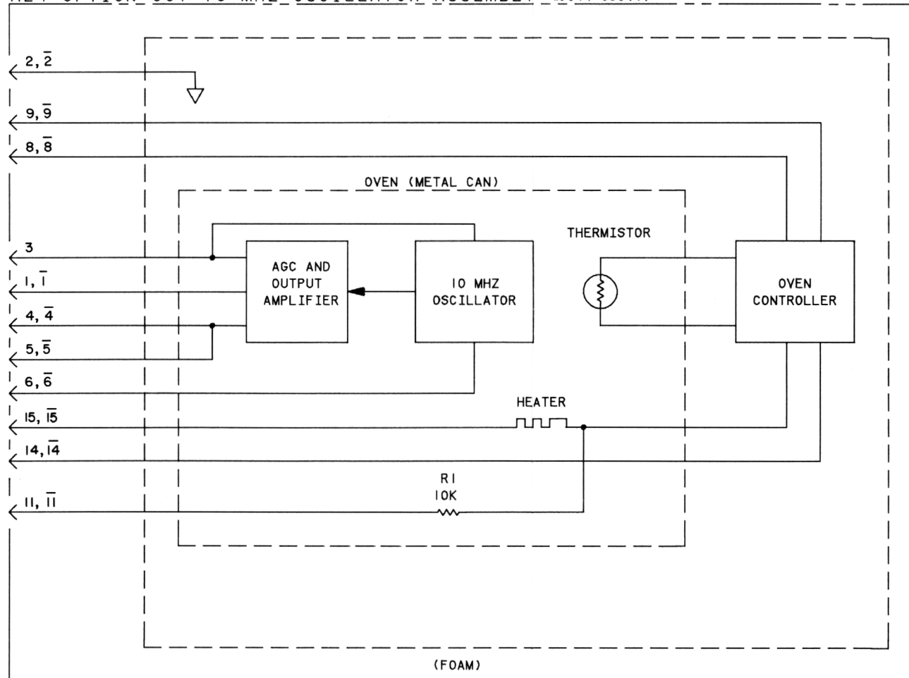
Figure 8-44. A24 Oscillator Assembly
