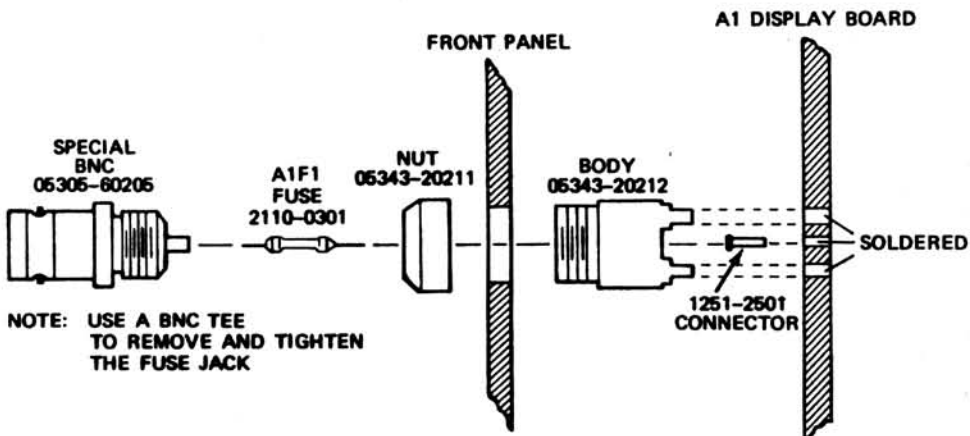
Figure 3. Front Panel Fuseholder for CHANGE 8
