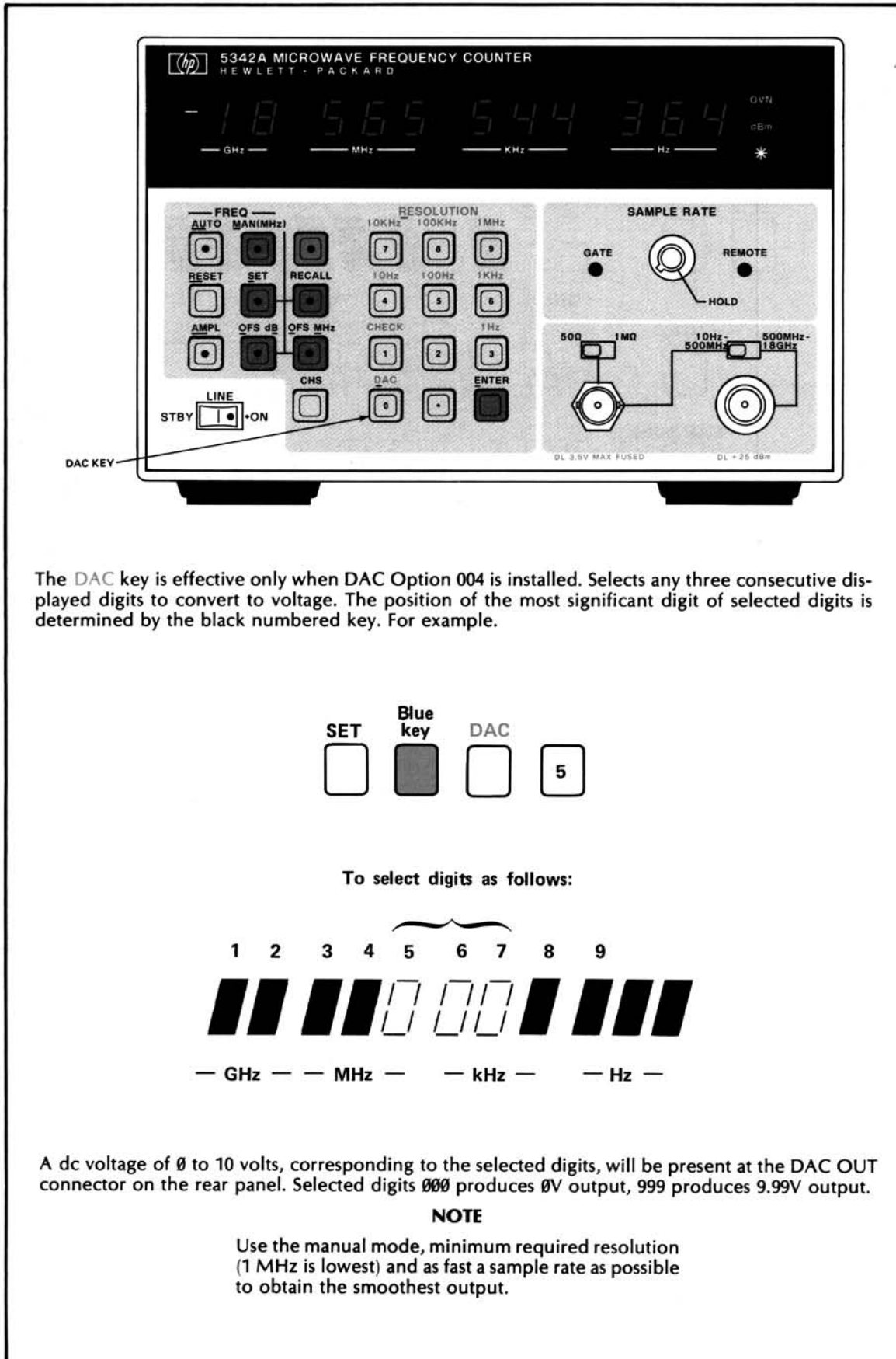
Figure 3-5. DAC Operation (Option 004)
