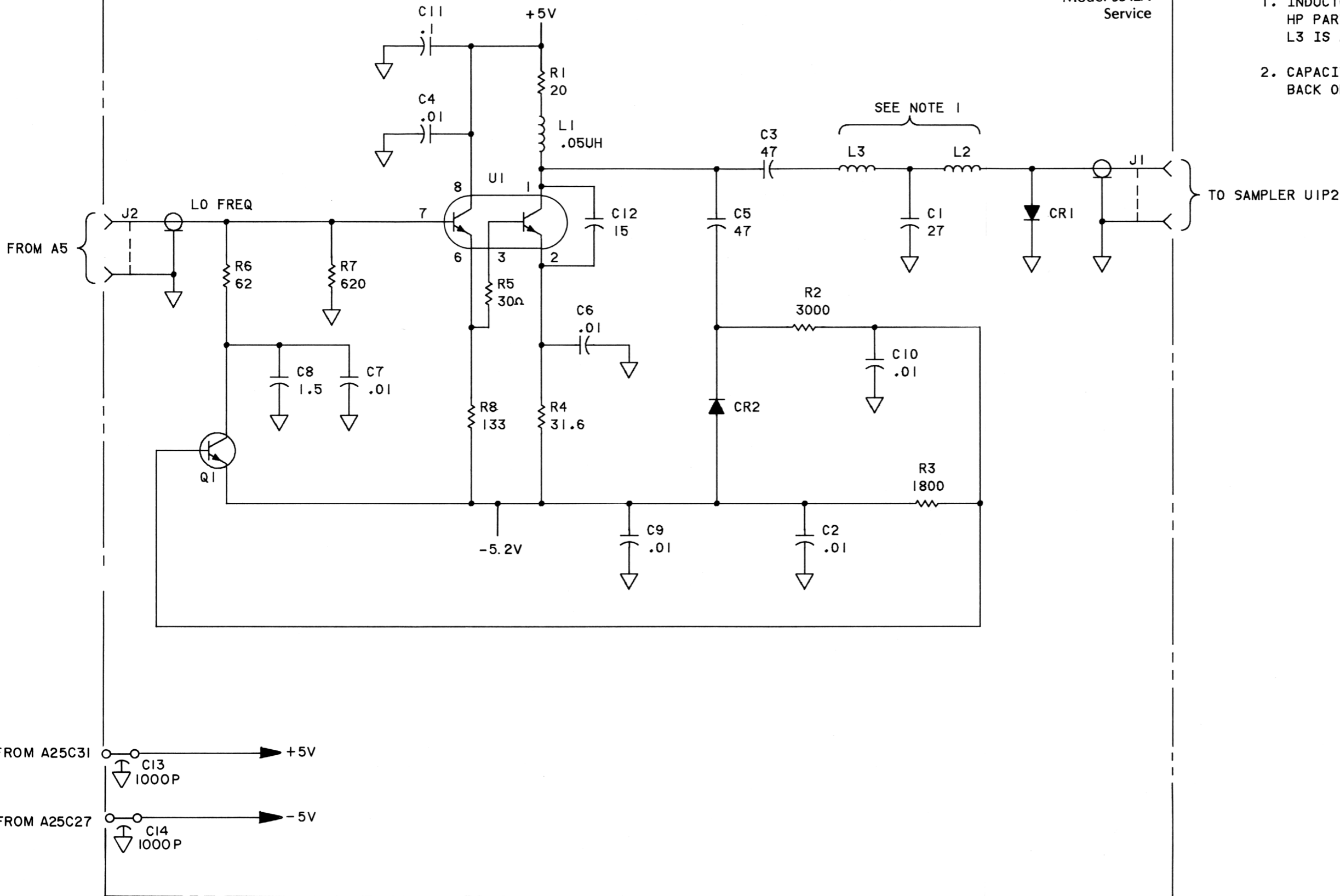
Figure 8-46. A26 Sampler Driver Assembly
